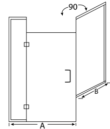
GG-1631-B Corner Enclosure with Buttress Return, Full Height Panels, and Wall Channels
