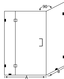
GG-1631 Corner Enclosure Open Above with Wall Clips (see clip pricing, pg 17)
