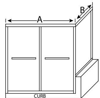
G-CS-1648-B Corner Shower Stall Enclosure with Buttress Return
