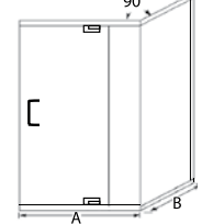
GAP-1631 Corner Enclosure with Header
