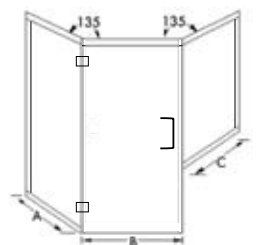
GG-1669-B Neo-Angle with Buttress Panel and Header
