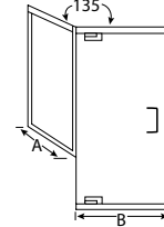
GAP-1669 2/3-B Two-Thirds Neo-Angle with Buttress Return and Header
