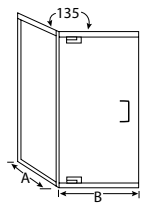
GAP-1669 2/3 Two-Thirds Neo-Angle with Header
