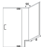
GAP-1631-B Corner Enclosure with Buttress Return and Header
