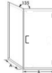
GW-1669-2/3 Two-Thirds Neo-Angle with Wall Channel
