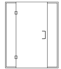
GG-1628 Full Height Panel, Door, Panel with Wall Channel
