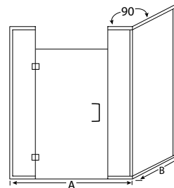
GG-1632 Corner Enclosure with Full Height Panels and Wall Channels
