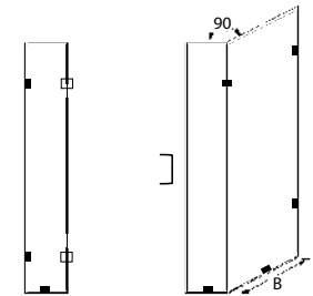
GG-1632 Corner Enclosure Open Above with Corner and Wall Clips (see clip pricing, pg 17)
