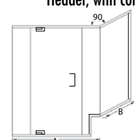
GAP-1632-B Panel, Door, Panel Corner Enclosure with Buttress Return and Header
