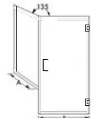
GW-1669-2/3-B Two-Thirds Neo-Angle with Buttress Panel and Wall Channel
