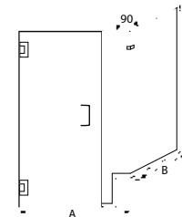
GW-1631-B Corner Enclosure with Buttress Return, Wall Channel & Corner Clip
